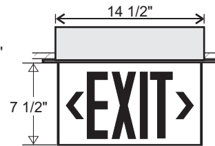
TOP MOUNT
